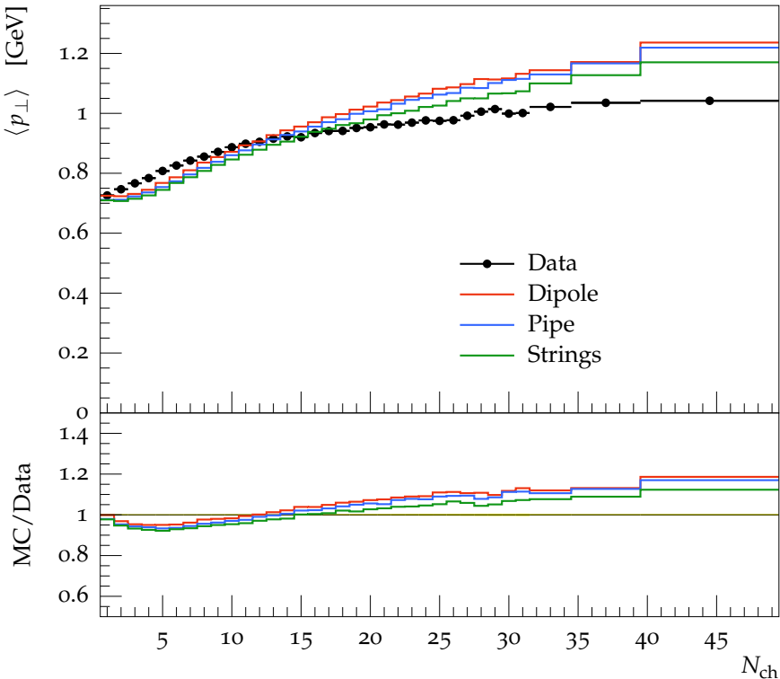
Charged \langle p_{\perp} \rangle vs. N_{\text{ch}} at 2760 GeV, track p_{\perp} > 500 MeV, for N_{\text{ch}} \geq
