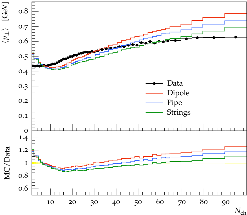
Charged \langle p_{\perp} \rangle vs. N_{\text{ch}} at 2760 GeV, track p_{\perp} > 100 MeV, for N_{\text{ch}} \geq
