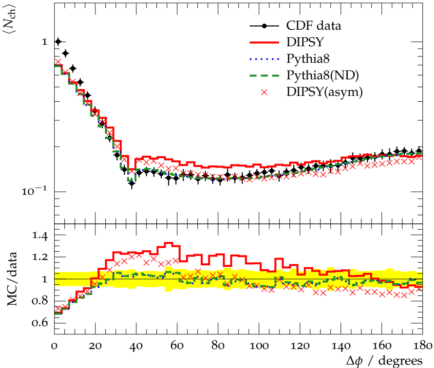
\langle N_{\text{ch}} \rangle vs. \Delta\phi from leading jet ( p_{\perp}^{\text{lead}} > 5 GeV)
