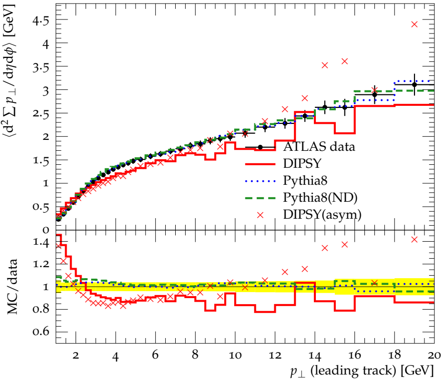
Away \Sigma p_{\perp} density vs. p_{\perp}^{\text{trk1}} , \sqrt{s} = 7 TeV, p_{\perp} > 100 MeV
