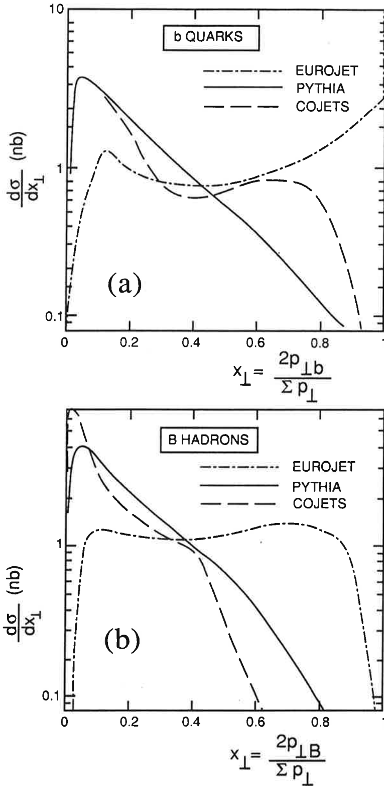
Figure 5: Inclusive transverse momentum fraction x_{\perp} for (a) b + \bar{b} quarks after perturbative treatment and (b) bottom hadrons after fragmentation. The total (parton level) transverse energy of the event is constrained to lie between 100 and 200 GeV.
