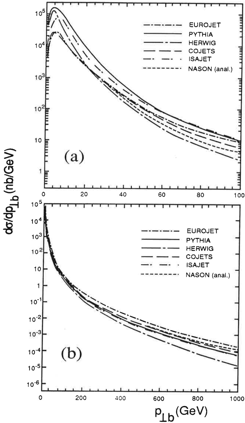
Figure 2: Inclusive b + \bar{b} transverse momentum distribution after the full perturbative treatment, i.e. shower or higher order matrix elements, at (a) low and (b) high transverse momentum p_{\perp} .
