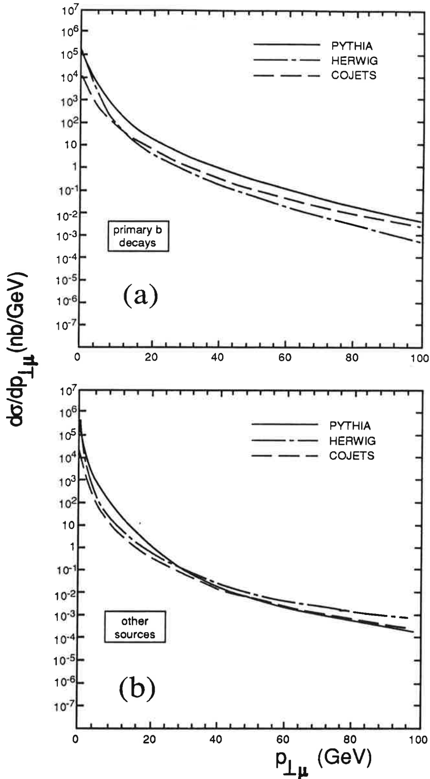
Figure 4: Inclusive muon p_{\perp} distributions, after full perturbative QCD, fragmentation and decay treatment. The direct muons from b + \bar{b} are shown in (a), whereas (b) shows the muons coming from other sources (from secondary b decays, or from charm production).
