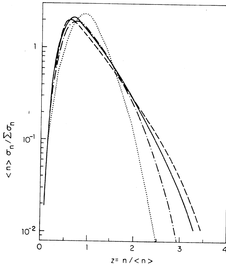
Figure 3: Scaled charged multiplicity distribution at 40 TeV, dash-dotted for solid sphere, full Gaussian, dashed exponential, dotted fixed impact parameter.
