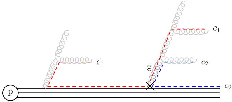
Figure 19: Example showing the colour flow produced by attaching the gluon g at the place indicated by the cross.
