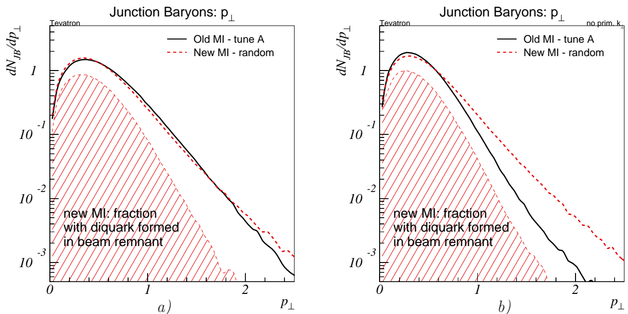
Figure 17: p_{\perp} spectra for junction baryons, a ) with primordial k_{\perp} switched on, and b ) with primordial k_{\perp} switched off. The shaded area represents the distribution in the new model of those junction baryons which arose by first forming a diquark in the beam remnant, cf. Section 4.2.
