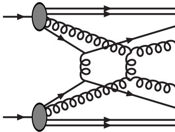
Figure 1: Schematic illustration of an event with two 2 \rightarrow 2 perturbative interactions.
