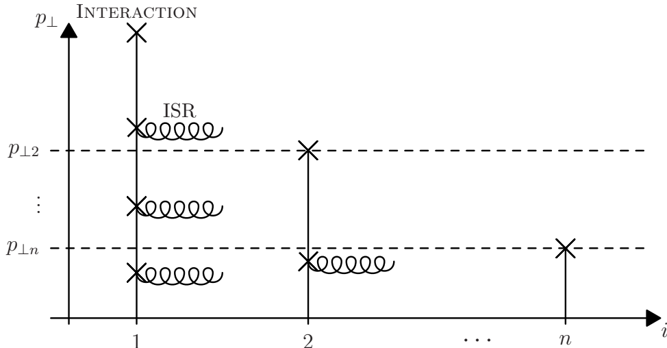
Figure 8: Schematic representation of the evolution of parton shower initiators in a hadron collision with n interactions (see text).
