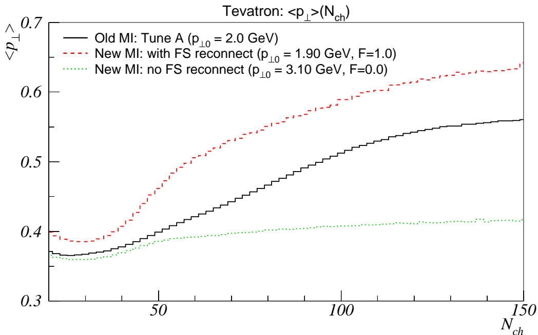
Figure 21: \langle p_{\perp} \rangle vs. n_{ch} at the Tevatron for Tune A (solid line), and for the new model with (dashed line) and without (dotted line) final-state reconnections allowed. Both of the new models use rapidity ordering of the colour lines in the initial state and give the same average charged multiplicity as Tune A, with the same impact parameter dependence as Tune A.
