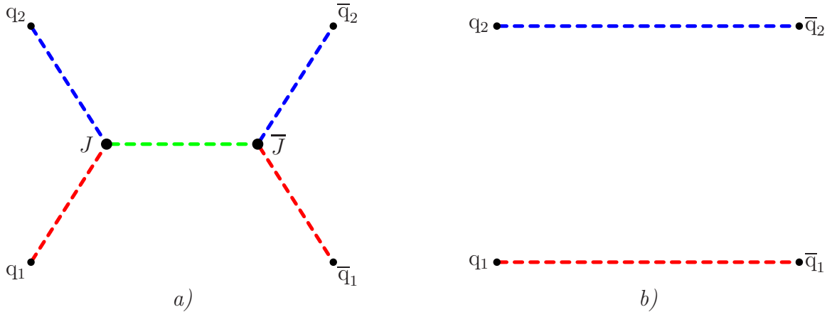
Figure 15: a) A string system (dashed lines) spanned between four quarks and containing a junction and an antijunction. b) The same parton configuration in colour space but with an alternative string topology. In a) the beam baryon numbers will still be present in the final state, while in b) they will have disappeared through annihilation.
