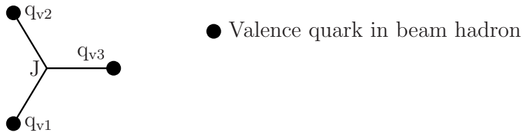
Figure 12: The initial state of a baryon, consisting of 3 valence quarks connected antisymmetrically in colour via a central ‘string junction’, J.
