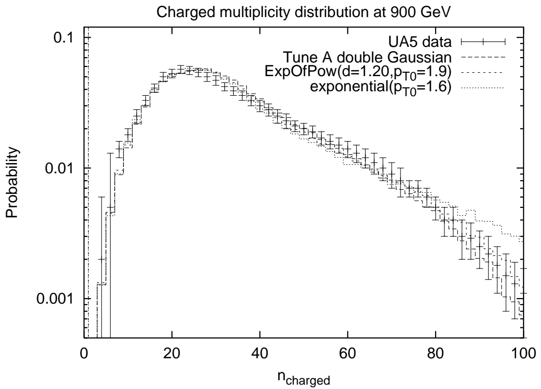
Figure 6: Charged multiplicity distribution at 200 and 900 GeV; different overlap profiles compared with UA5 data [46].
