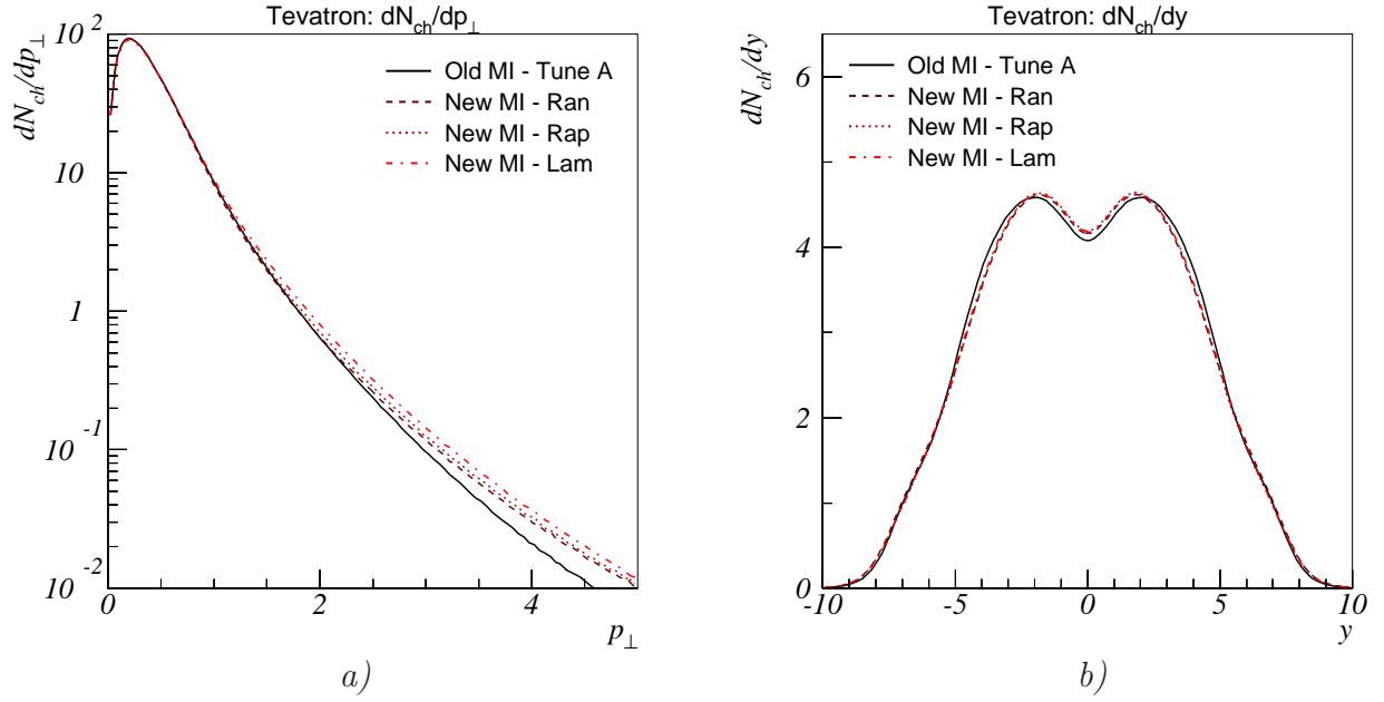
Figure 24: Charged particle p_{\perp} and y spectra at the Tevatron. Results are shown for Tune A (solid), Ran (dashed), Rap (dotted), and Lam (dash-dotted), as defined in Table 1.
