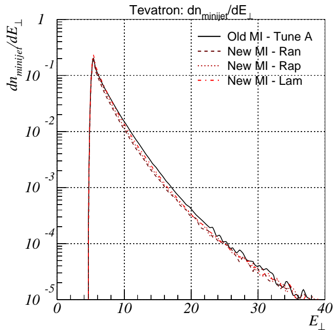
Figure 23: The number of jets as a function of jet E_{\perp} (for E_{\perp} > 5\text{GeV} ) in min-bias collisions at the Tevatron. Results are shown for Tune A (solid), Ran (dashed), Rap (dotted), and Lam (dash-dotted), as defined in Table 1.
