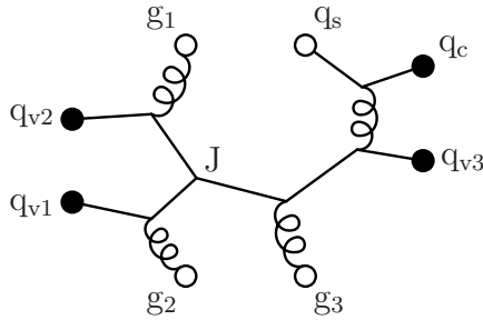
Figure 16: Example of how a given set of parton shower initiators could have been radiated off the initial baryon valence configuration, in the case of the ‘purely random’ correlations discussed in the text. In this example, the baryon number is disconnected from the beam remnant. Instead, it is the final-state partons connected to the colour lines of g_1 , g_2 , and g_3 which determine how the junction moves and hence how the baryon number flows in the event.
