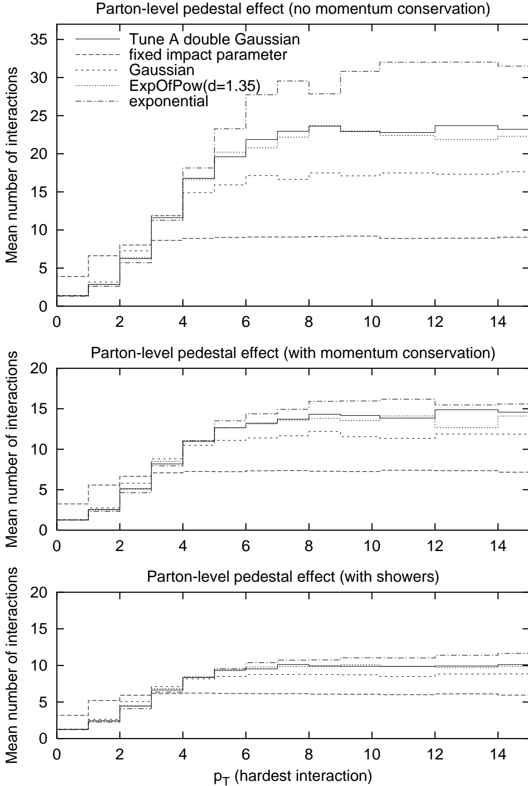
Figure 5: Average number of interactions as a function of the p_{\perp} of the hardest interaction, for p\bar{p} at 1.8 TeV, top without momentum conservation constraints, middle with such constraints included but without (initial-state) showers, and bottom also with shower effects included.
