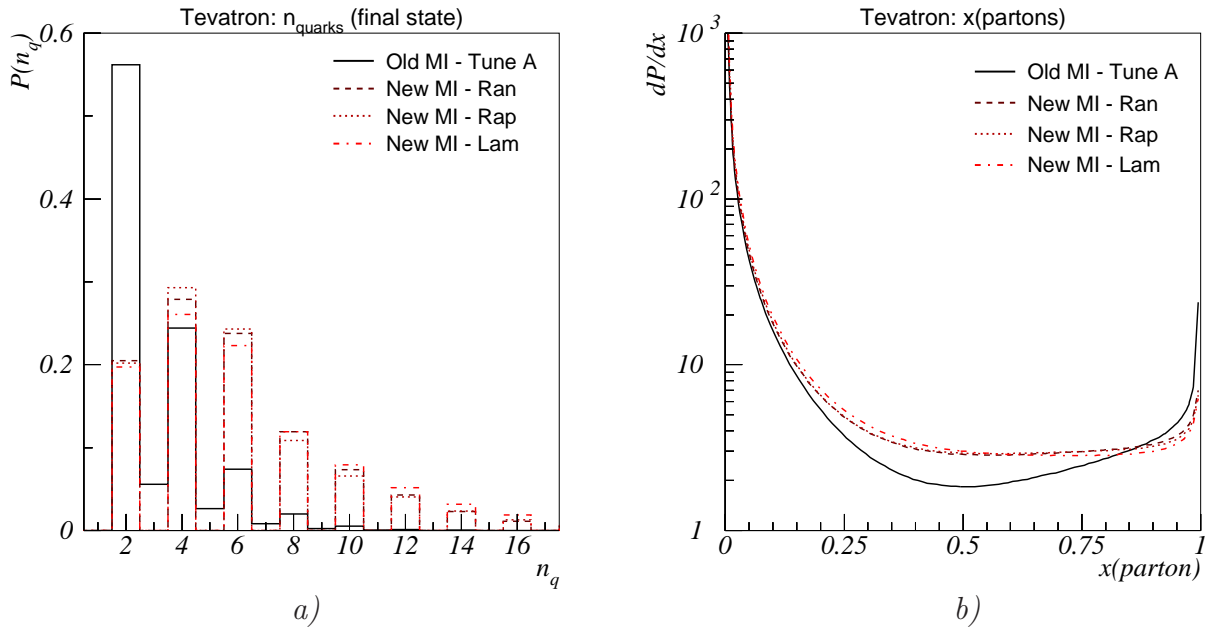
Figure 25: a ) Number of final-state quarks (not counting diquarks) and b ) final-state parton x values at the Tevatron. Results are shown for Tune A (solid), Ran (dashed), Rap (dotted), and Lam (dash-dotted), as defined in Table 1.
