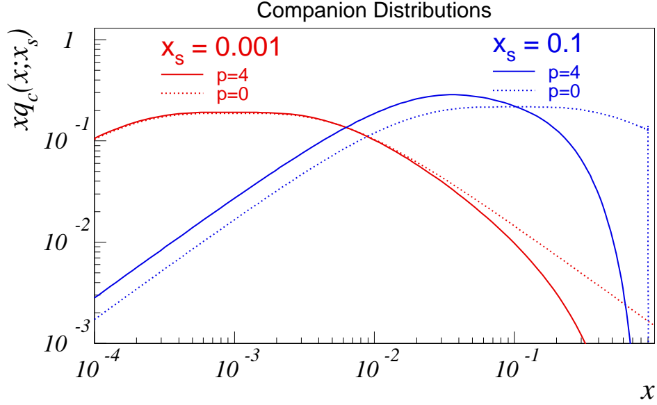
Figure 9: Companion distributions for p = 4 (solid lines) and p = 0 (dotted lines), for two different values of x_s .
