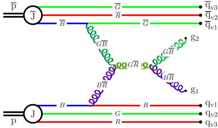
Figure 14: Example of colour assignments in a p\bar{p} collision, with explicit colour labels shown on each propagator line. Note that the blue colour line starting on the junction J is connected via the colour flow of the hard scattering to the antiblue colour line of \bar{J} .
