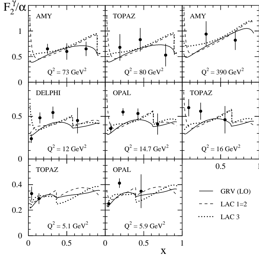
Figure 3: Recent data on F_2^\gamma(x, Q^2) from TRISTAN [23, 24] and LEP [25, 26] compared to the LO fits to all previous data of LAC [19] and GRV [14].
