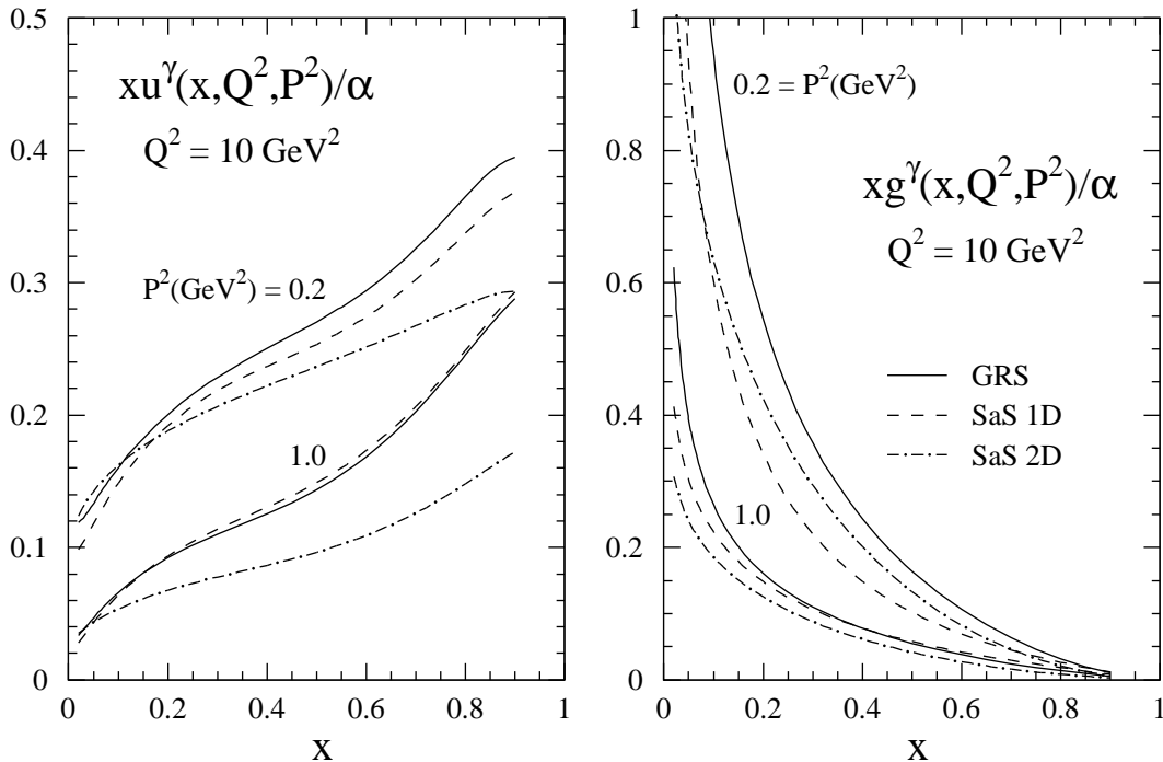
Figure 4: The u -quark and the gluon distributions of the virtual photon in LO as suggested in refs. [17, 35] at two selected values of the photon virtuality P^2 .
