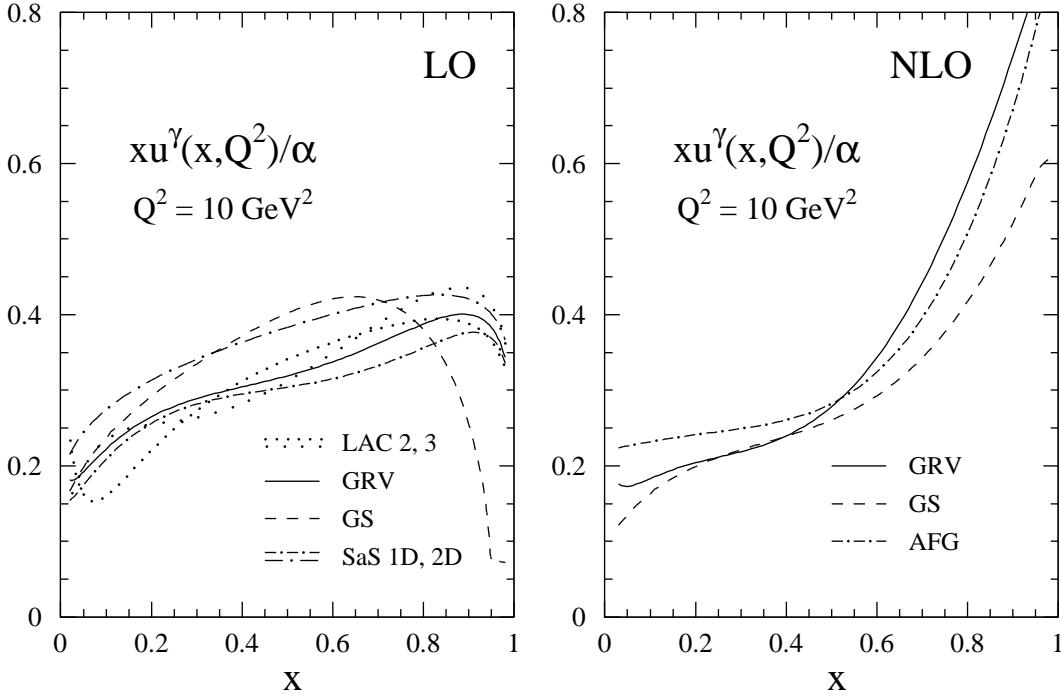
Figure 1: Photonic u -quark parametrizations at LO [14, 17, 19, 20] and NLO [14, 16, 20]. The NLO results are presented in the \overline{\text{MS}} scheme. For a discussion of the different assumptions and F_2^\gamma data sets employed see [5].
