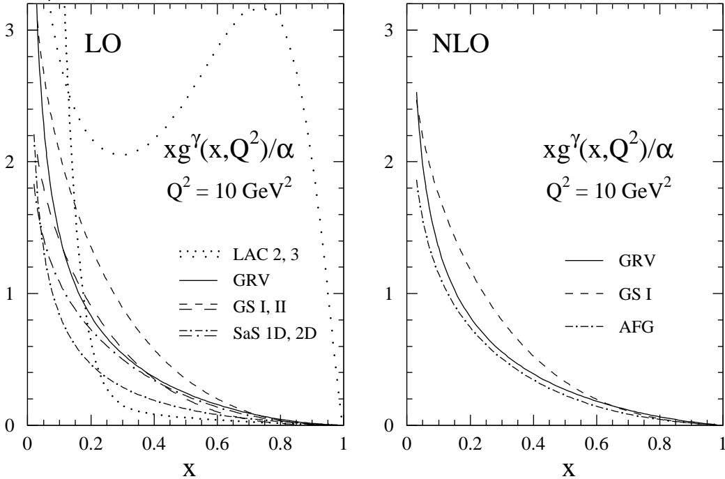
Figure 2: Parametrizations of the photon's gluon distribution at LO [14, 17, 19, 20] and NLO [14, 16, 20]. Note that the similarity of the NLO results is due to common VMD prejudices and not enforced by data.
