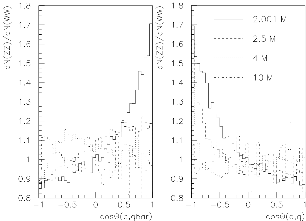
Figure 4: The ratio of angular distributions in the Z^0Z^0 and W^+W^- events, at different multiples of the respective gauge boson mass, and without any Breit-Wigner broadening (in order to let low masses correspond to bosons almost at relative rest). Left frame: between a quark from one boson and an antiquark from the other. Right frame: between the quarks or the antiquarks.
