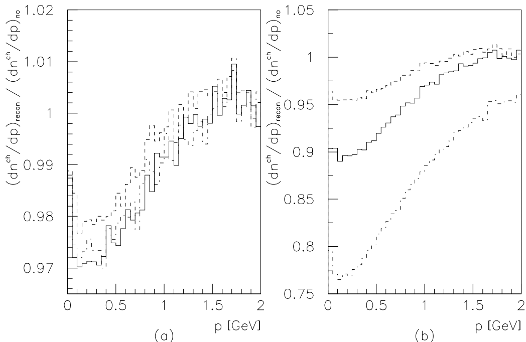
Figure 1: Depletion of low-momentum particles in some realistic (left) and toy (right) scenarios [8].
