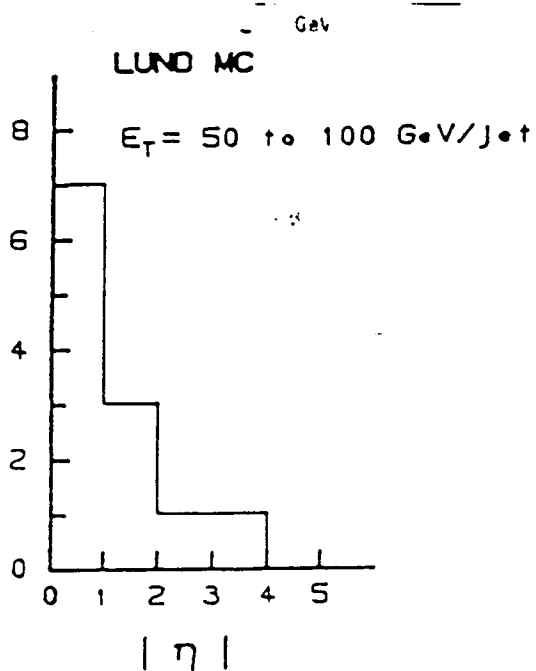
Fig. 9 a) Rapidity distribution for jets with E_T > 100 \text{ GeV} other than the hard scattering jets as generated by the LUND Monte Carlo for \sqrt{s} = 40 \text{ TeV} pp interactions. b) Same as 9a but for jets with E_T = 50 \text{ GeV} .
