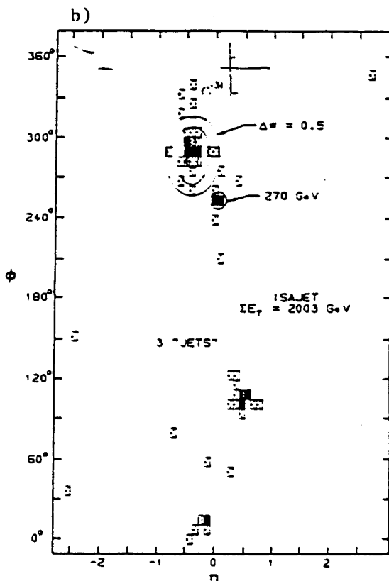
Fig. 5: a) Typical high E_T event from a 2 to 2 hard scattering interaction as generated by the ISAJET at \sqrt{s}=40 TeV and displayed in the \eta, \phi projection. This event appears to be a two or three jet event using the jet criteria described in the text. b) Another "typical" 2 to 2 high E_T event as described above except that there appear to be three substantial jets. The \Delta\omega = \sqrt{(\Delta\eta)^2 + (\Delta\phi)^2} = 0.5 contour indicates the area that a "reasonable" jet algorithm might assume for a jet size. c) Typical 2 to 2 high E_T event as described above which appears to have 5 or 6 substantial jets.
