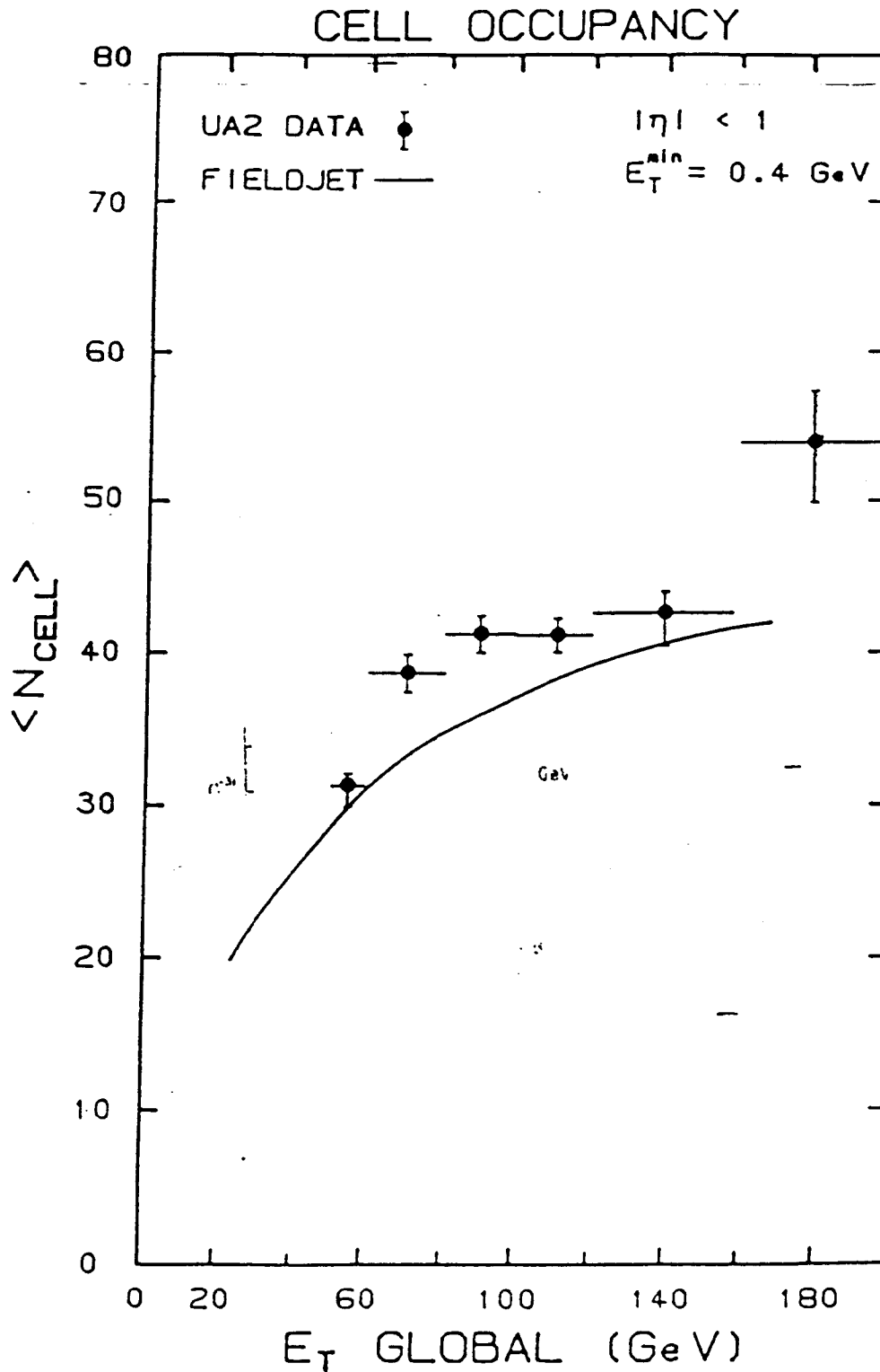
Fig. 4 Predicted occupancy of detector cells of size \Delta\eta = 10 \times 15^\circ from FIELDJET compared to data of UA2 at \sqrt{s} = 540 \text{ GeV} as a function of global E_T . A cell is considered to be occupied if E_T within that cell is greater than 0.4 \text{ GeV} .
