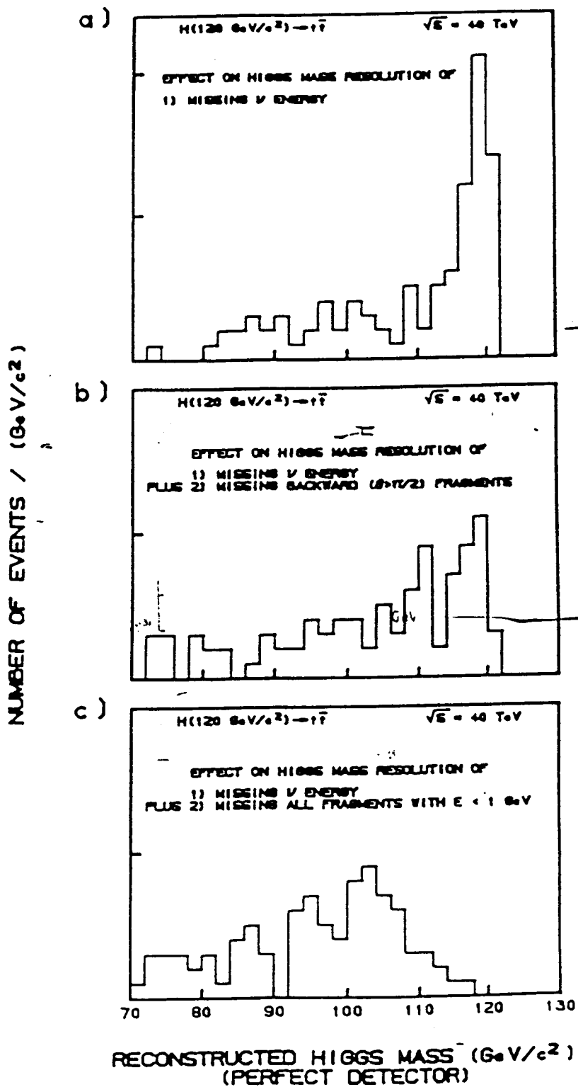
Fig. 16 a) Effect of missing neutrinos from top quark decay on the reconstruction of the mass of Higgs \rightarrow t\bar{t} at \sqrt{s}=40 \text{ TeV} for 120 \text{ GeV}/c^2 Higgs. b) Combined effect of missing neutrinos and missing energy in the reconstruction of the Higgs mass. c) Combined effect of missing neutrinos and omission of all E < 1 \text{ GeV} fragments from the t quark jets on the reconstruction of the Higgs mass.
