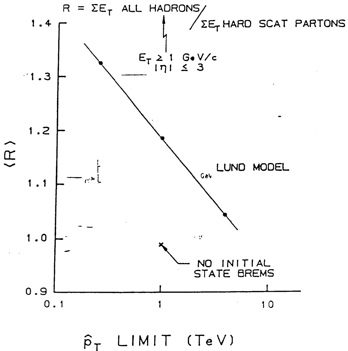
Fig. 7 Ratio of the E_T in \sqrt{s}=40 TeV interactions generated by the LUND Monte Carlo to E_T in the hard scattered parton jets as a function of \hat{p}_T for the hard scattering process.
