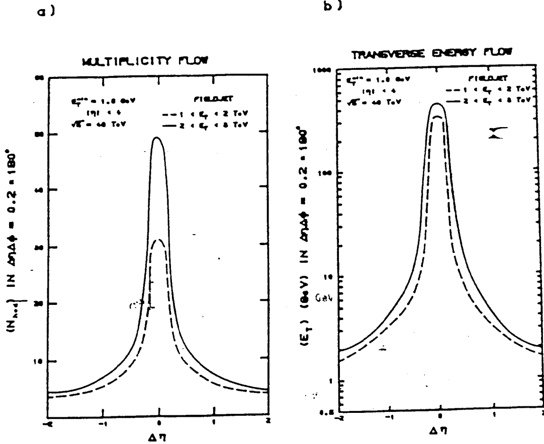
Fig. 13 a) Charged particle multiplicity flow as predicted by FIELDJET at \sqrt{s} = 40 TeV for global E_T less than 2 TeV and for global E_T between 2 and 3 TeV.
