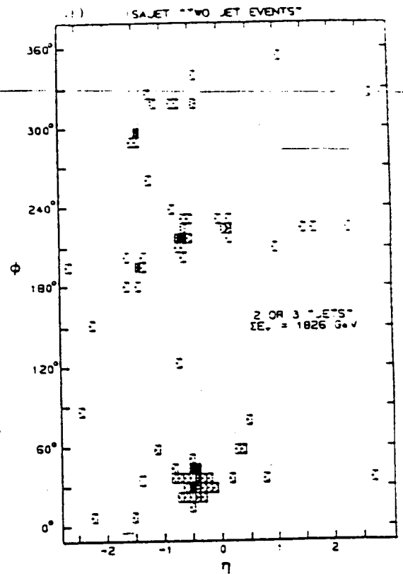
Fig. 5: a) Typical high E_T event from a 2 to 2 hard scattering interaction as generated by the ISAJET at \sqrt{s}=40 TeV and displayed in the \eta, \phi projection. This event appears to be a two or three jet event using the jet criteria described in the text. b) Another "typical" 2 to 2 high E_T event as described above except that there appear to be three substantial jets. The \Delta\omega = \sqrt{(\Delta\eta)^2 + (\Delta\phi)^2} = 0.5 contour indicates the area that a "reasonable" jet algorithm might assume for a jet size. c) Typical 2 to 2 high E_T event as described above which appears to have 5 or 6 substantial jets.
