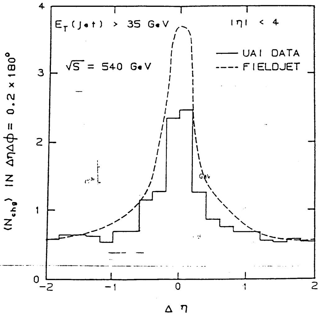
Fig. 11 Charge particle multiplicity flow relative to the highest E_T jet in pp collisions at \sqrt{s}=540 GeV with |\eta| < 4 and E_T(\text{jet}) > 35 GeV. Cell size of \Delta\eta\Delta\phi = 0.2 \times 180^\circ has been used. The data is that of the UAI experiment and the prediction is that of FIELDJET.
