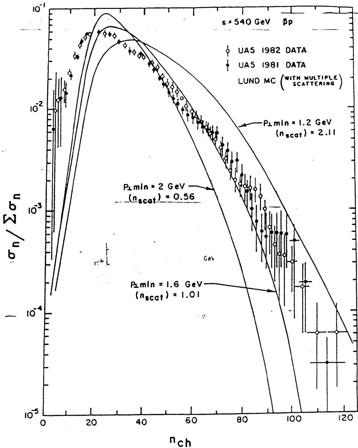
Fig. 3 Charged particle multiplicity distributions at \sqrt{s}=540 \text{ GeV} as measured by UA5. The predictions of the LUND Monte Carlo including the incorporation of multiple interactions between different pairs of partons in the beam hadrons. Three predictions for different P_{\perp \text{ MIN}} cutoffs are shown along with the number of multiple interactions that these cutoffs correspond to.
