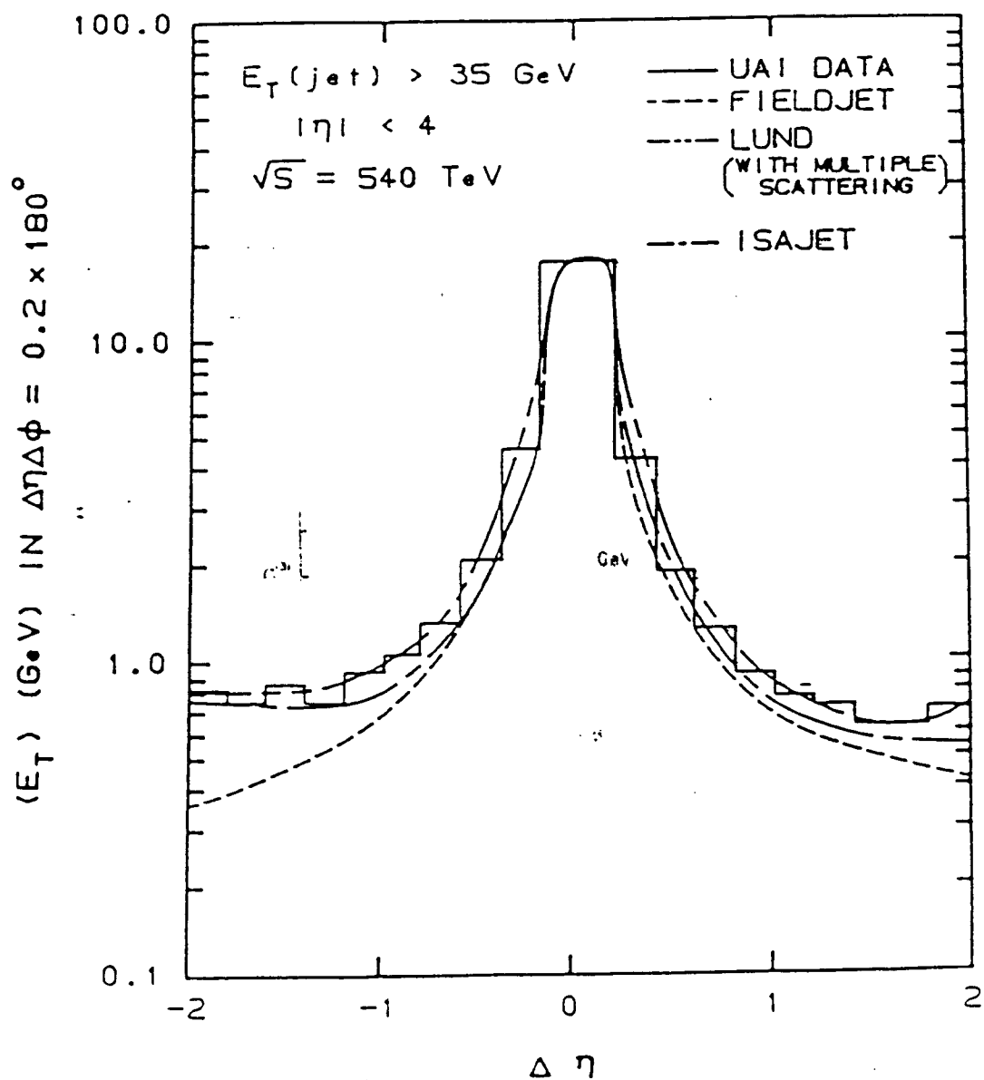
Fig. 12 Transverse energy flow with the same conditions as those of Fig. 11. The data is from UAI and the predictions are those of FIELDJET, ISAJET, and LUND.
